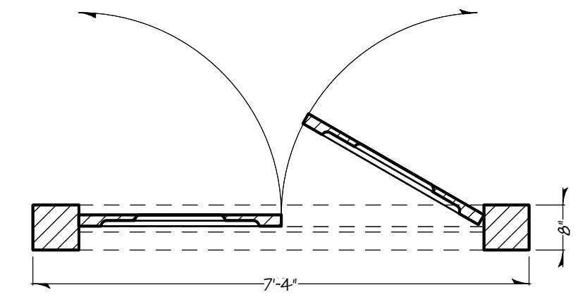
DOOR UNIT PLAN VIEW
