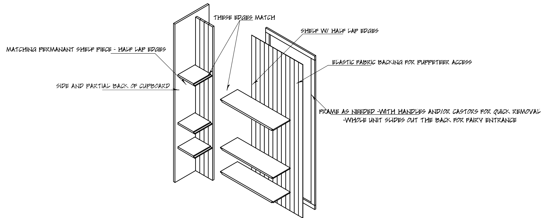
REMOVABLE SHELF UNIT- EXPLODED VIEW
