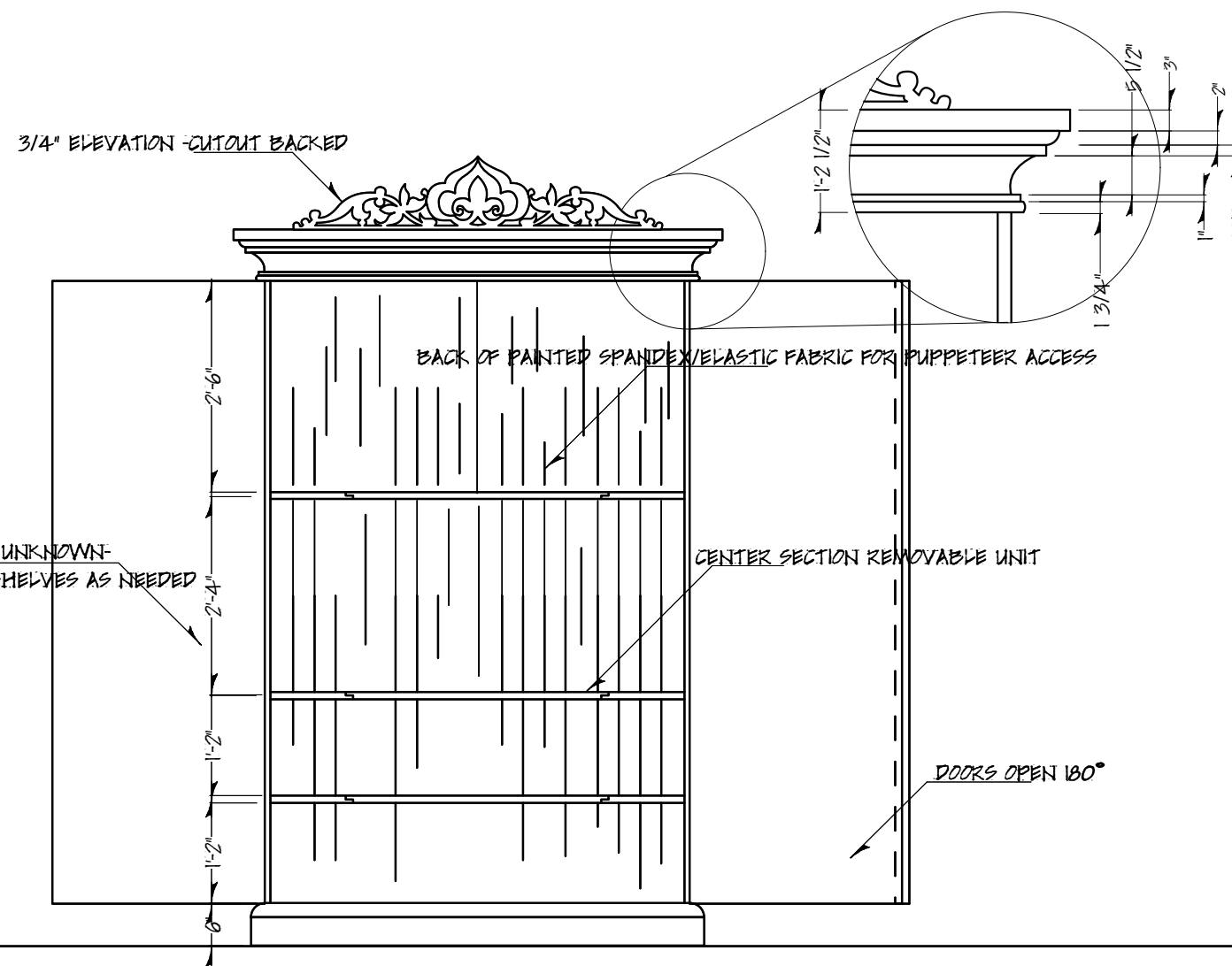
TOY CUPBOARD FRONT EL.- DOORS OPEN
