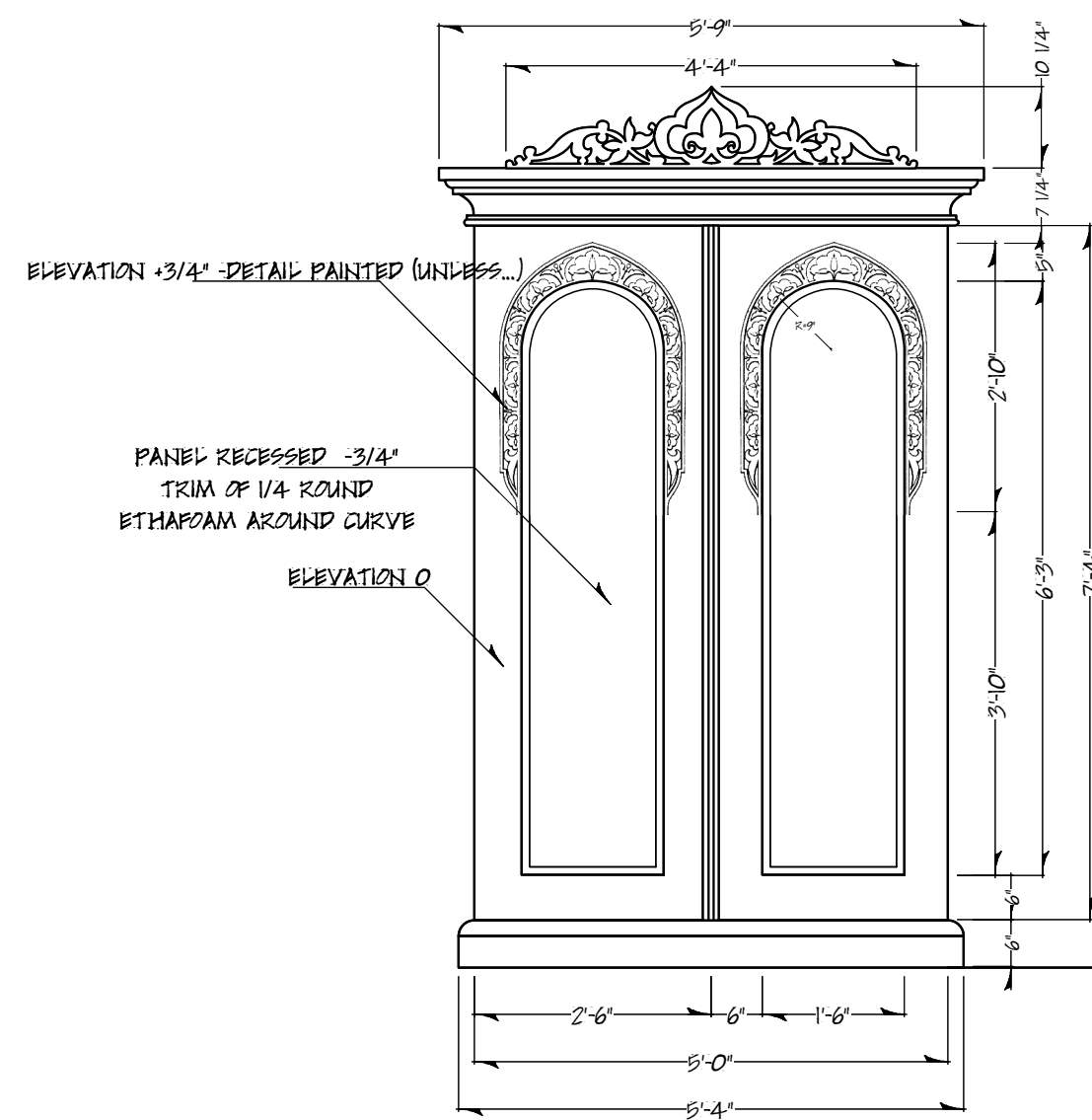
TOY CUPBOARD FRONT ELEVATION
