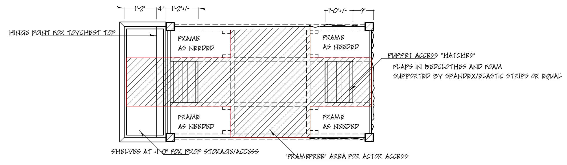
BED/TOYCHEST UNIT- PLAN VIEW
