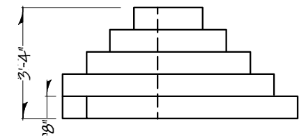
GARDEN STEPS FRONT ELEVATION
