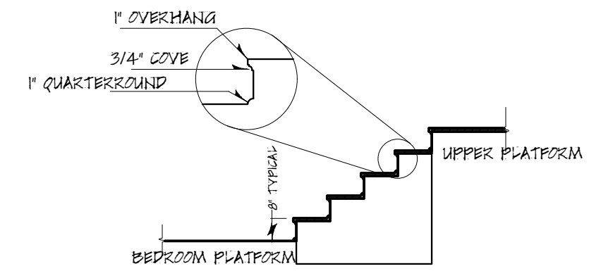
SECTION C-C
