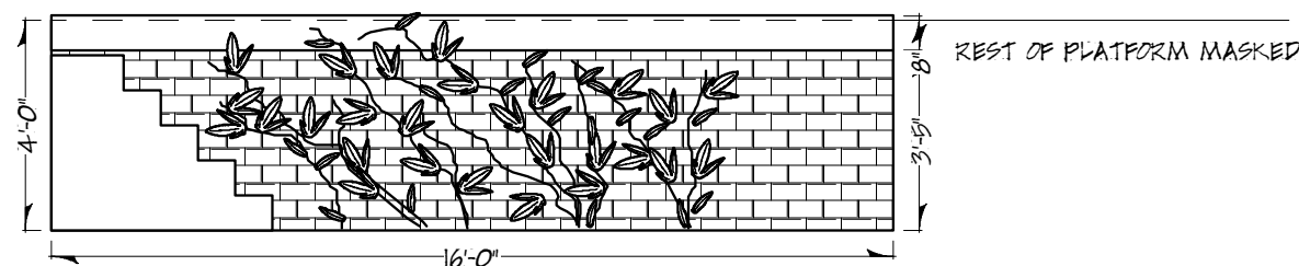
FACING "H" FRONT ELEVATION
